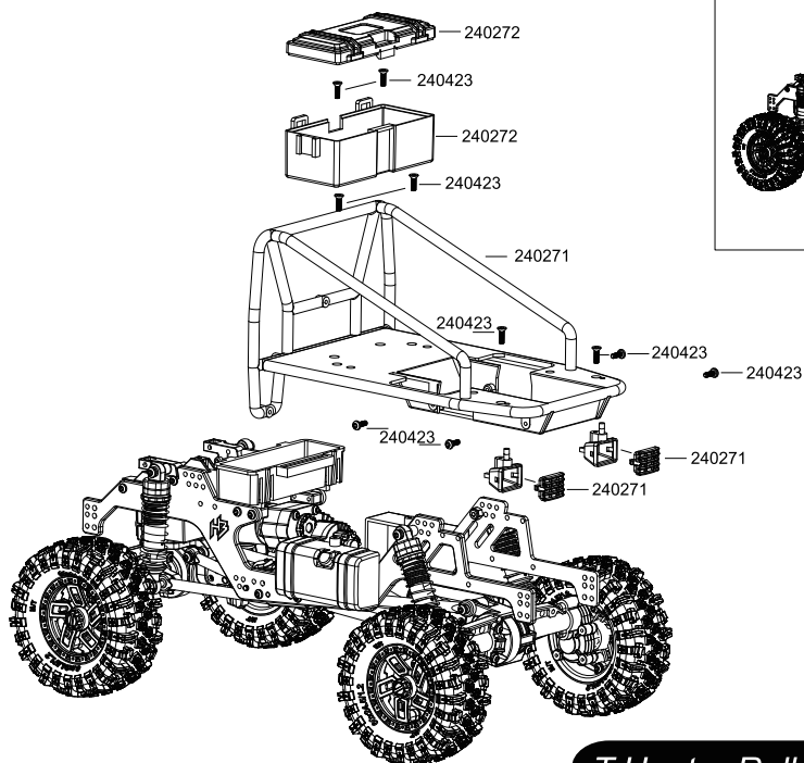
T-Hunter Rollcage Installation
