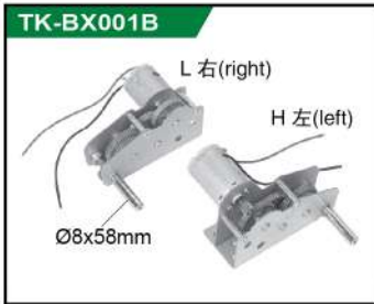
TK-BX001B 金属齿轮驱动箱(钢质齿轮) Metal gear drive box (Steel gear)
